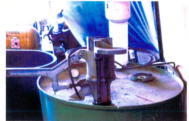
Use an aerosol can puncturing device, for example this one mounted over a hazardous waste drum, to safely drain the contents of your aerosol cans
